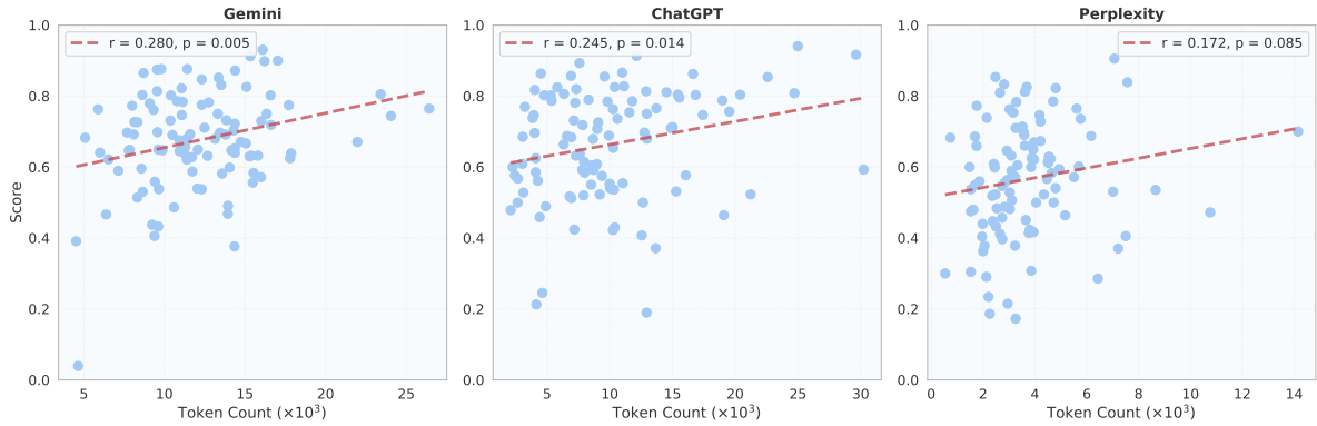
Figure 7: Comparison of length vs. score across token count for the ternary setting.
